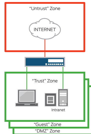
Figure 1: Firewalls, zones and policies
